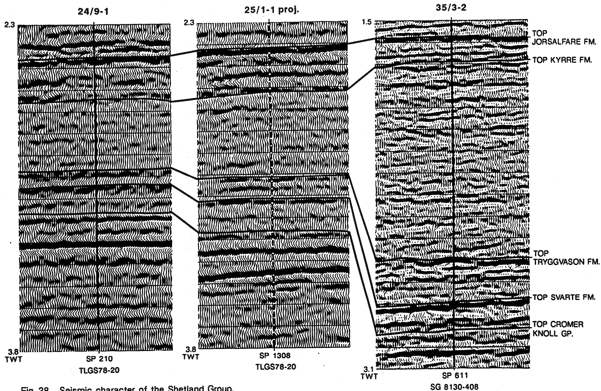
Fig. 38 Seismic character of the Shetland Group.
