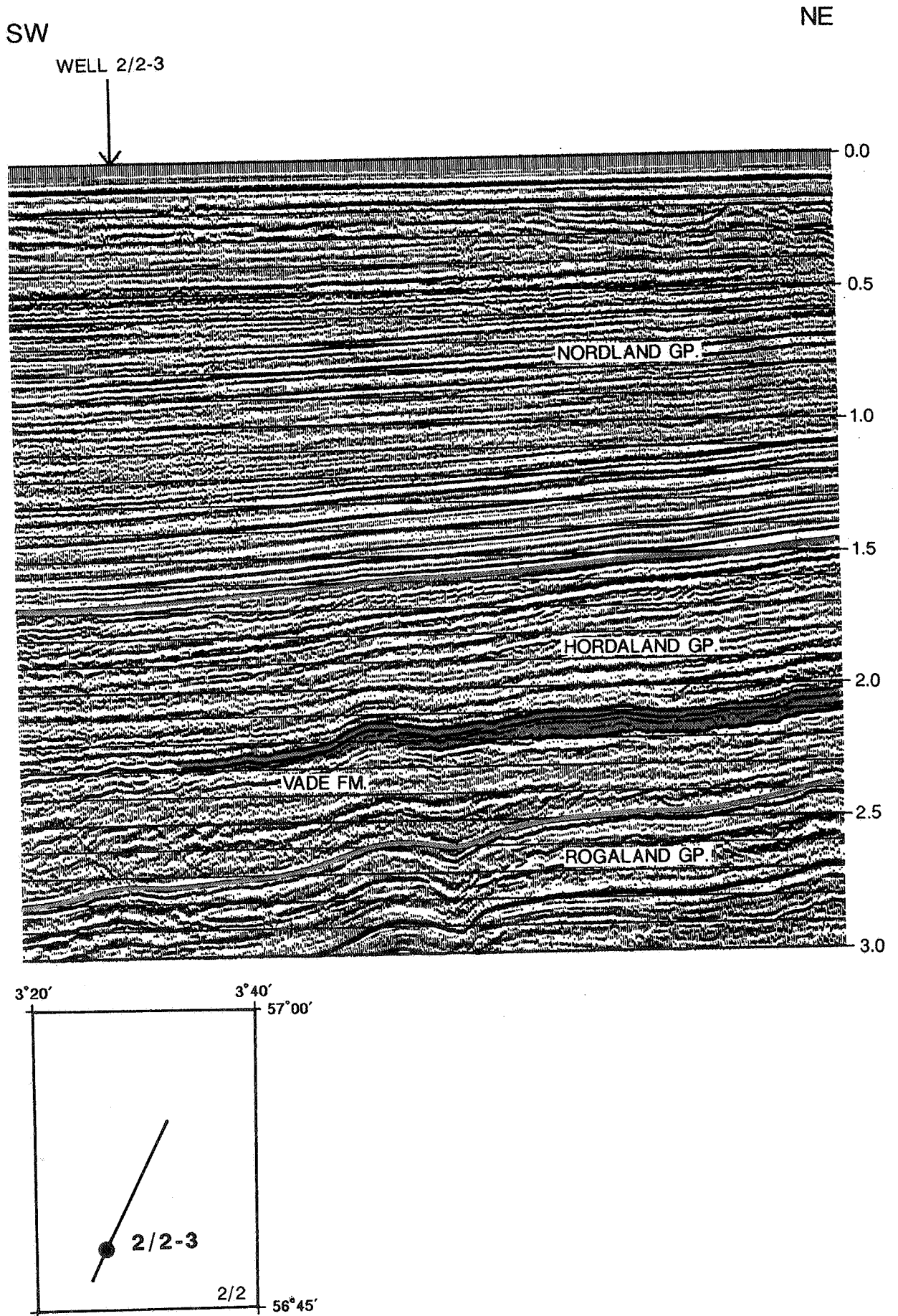
Fig. 69 Seismic section showing Hordaland Group with Vade Formation and Nordland Group.
