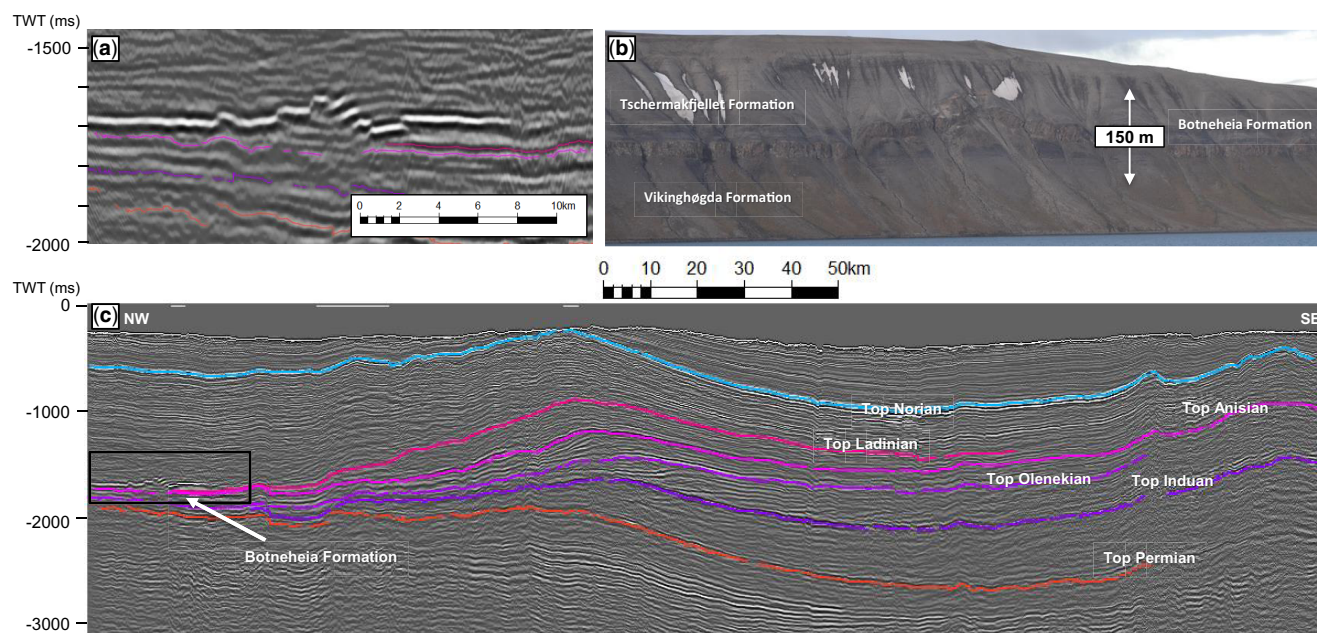
Fig. 7. Igneous intrusions in the North Barents CTSE. The igneous sills occur on the downslope part of clinoform bottomsets where organic-rich shales are assumed to be present. Outcrops on the northwestern Edgeøya on Svalbard, where a sill penetrates the soft shales of the Middle Triassic Botneheia Formation, have a similar configuration. Note the similar geometry of the cropping-out intrusion compared to the seismic example. The regional seismic interpretation indicates the presence of clinoform sequences in the Triassic succession.
