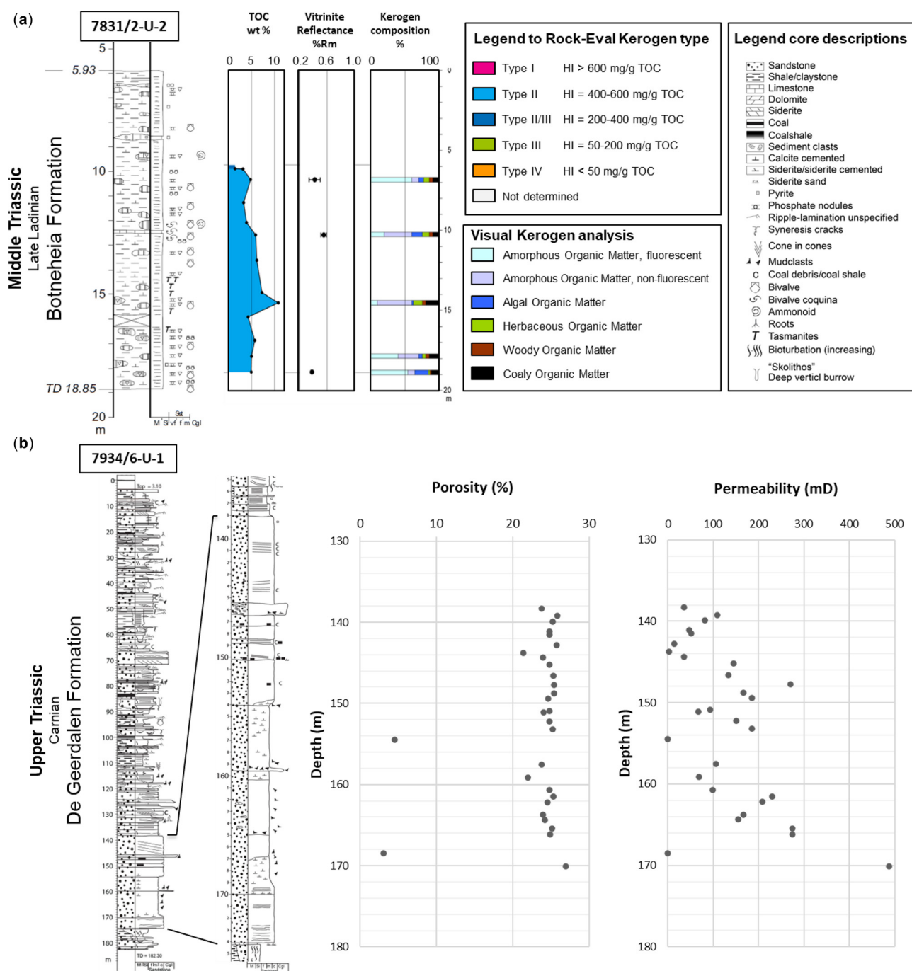
Fig. 10. (a) The organic-rich source rock assigned to the Steinkobbe/Botneheia Formation in 7831/2-U-2 on the Kong Karl platform. (b) Channel sandstones with good reservoir properties in core 7934/6-U-1 offshore Kvitøya.
