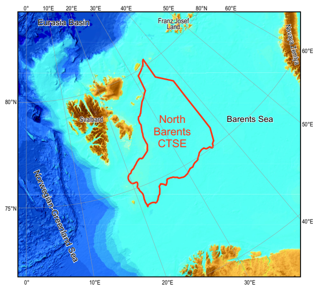
Fig. 1. Overview and location of the North Barents Composite Tectono-Sedimentary Element (CTSE).
