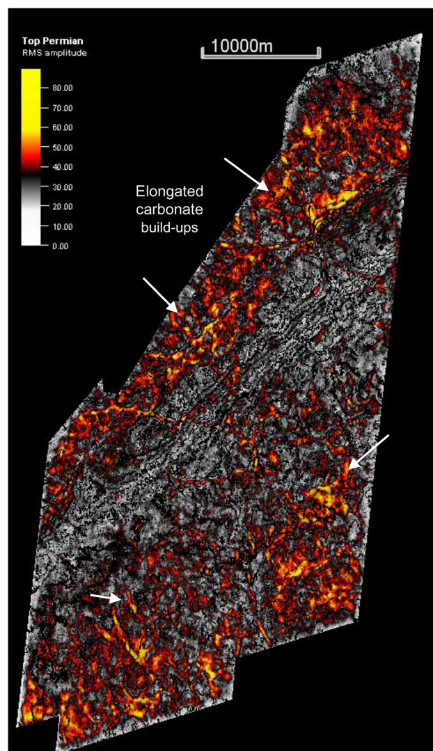
Fig. 11. RMS amplitude map from the Top Permian surface on the eastern parts of the Sentralbanken high, showing a network of elongated carbonate build-ups. The location of 3D seismic survey NPD19001 is shown in Figure 2.
