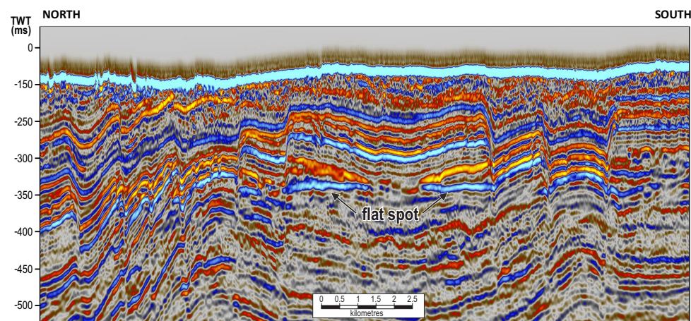
Fig. 8. Seismic line NPD1301R17-HR-222 showing a prominent flat spot in Jurassic reservoirs in several shallow fault blocks on the Storbanken high.
