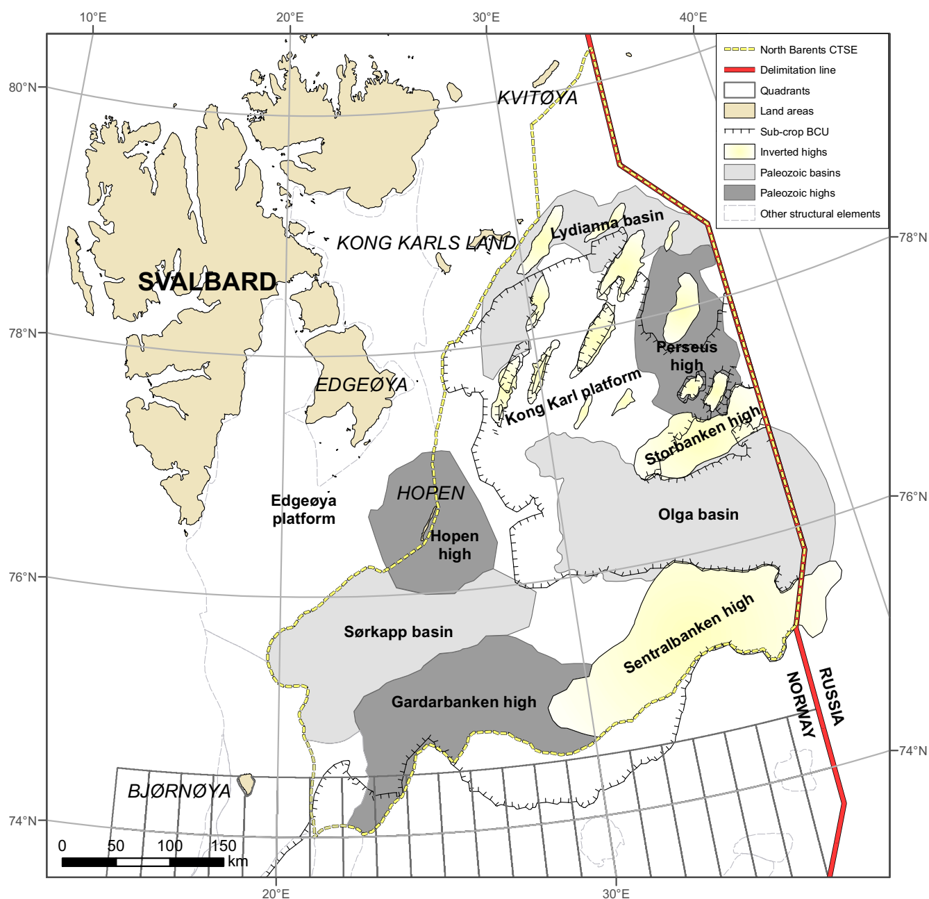
Fig. 3. The structural elements within the North Barents Composite Tectono-Sedimentary Element.
