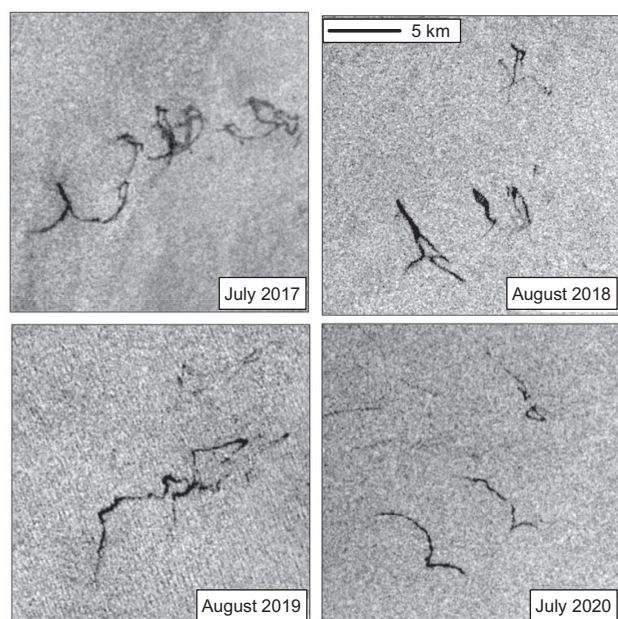
Fig. 9. Large oil slicks visible on SAR satellite images over the same area of the Sentralbanken high in 2017, 2018, 2019 and 2020. Source: Copernicus Sentinel data 2017–20, processed by the European Space Agency.
