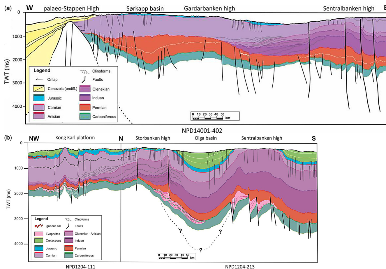
Fig. 6. (a) Regional east–west-orientated geoseismic profile across the Sentralbanken high, Sørkapp basin and palaeo-Stappen High. Note the westwards thinning of the Lower–Middle Triassic clinoform sequences and the onlapping of the Upper Triassic succession towards the palaeo-Stappen High. The Sentralbanken high is characterized by a Paleozoic core with horst and graben structures formed in the Mississippian, and small- and large-scale faults that extend towards and crop out at the seafloor. The Sørkapp basin is dominated by a thick succession of Carboniferous and Permian sediments, and the westernmost part of the profile is dominated by a thick Cenozoic succession. The location of the profile is shown in Figure 2. (b) Regional south–north- and NW-orientated geoseismic profiles across the Sentralbanken high, Olga basin, Storbanken high and Kong Karl platform. The Paleozoic successions consist mostly of carbonates and evaporites that form salt anticlines and bodies, and are faulted close to the Sentralbanken high. On the Storbanken high, large faults detach into the salt structure. The Triassic consists of clinoform sequences that become gradually thinner and younger towards the NW. The Jurassic succession is thin and thoroughly faulted. Note also the thinning of the Cretaceous succession towards the highs and deepening into basins, which suggests that these were structural highs during the formation of the Olga basin. The approximate base of the Olga basin is also indicated. The location of the profile is shown in Figure 2. TWT, two-way travel time.
