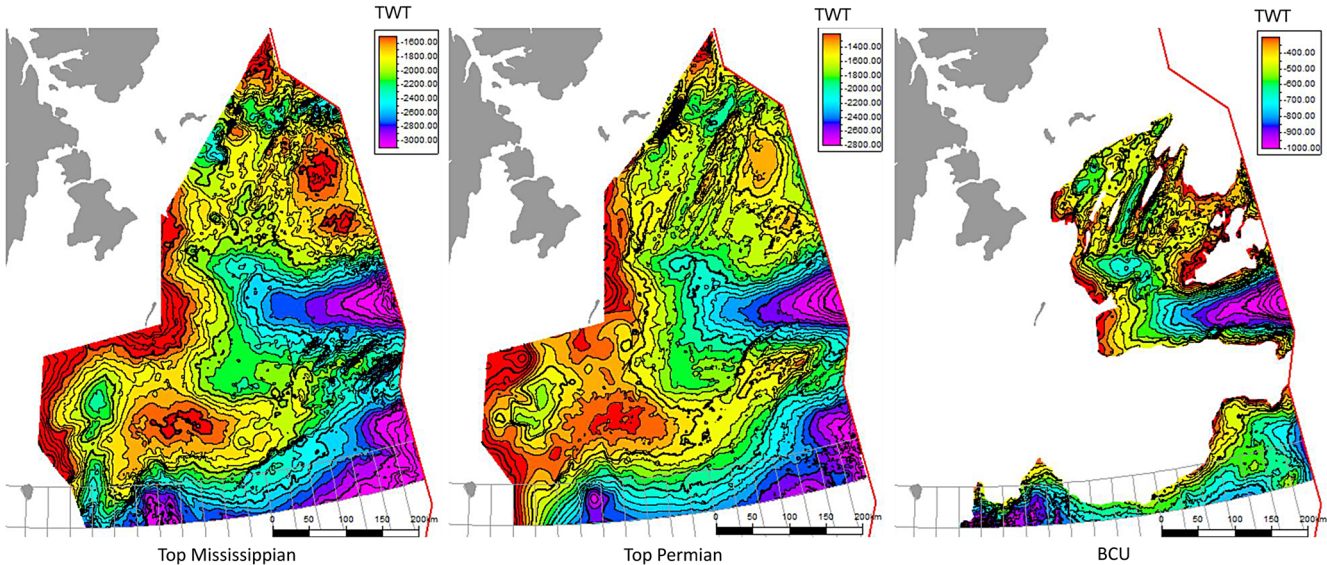
Fig. 5. Structural time maps for the Top Mississippian, Top Permian and Base Cretaceous Unconformity (BCU) in the North Barents Composite Tectono-Sedimentary Element. TWT, two-way travel time (ms).
