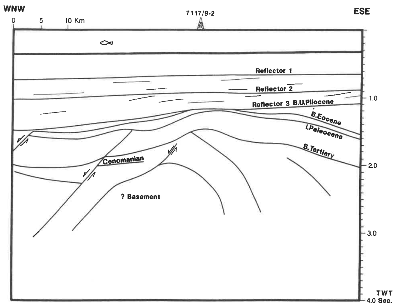
Fig. 7. Geoseismic section through Hole 7117/9-2.
