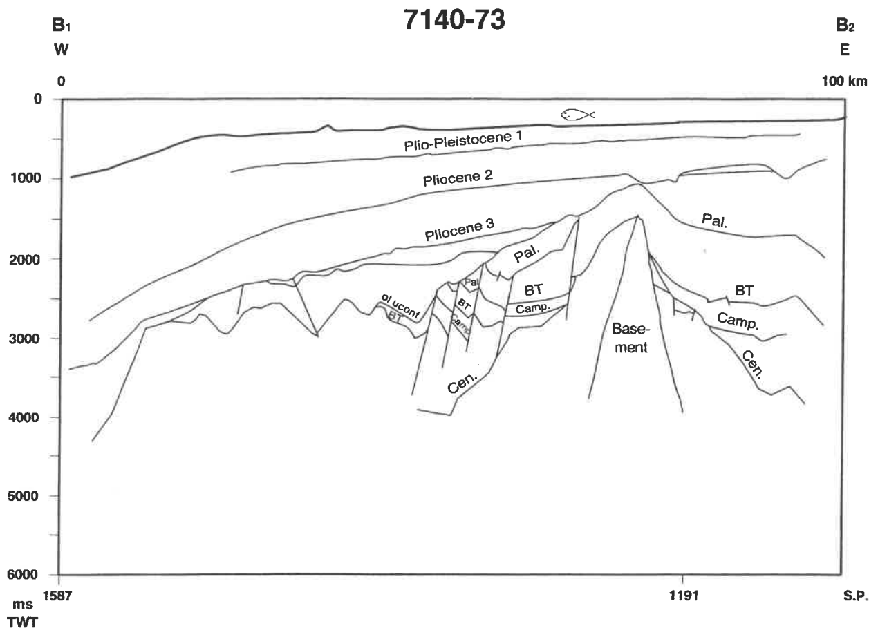
Fig. 5. Geoseismic section from the shelf edge into the wedge. The location of the line is shown on Fig. 2.
