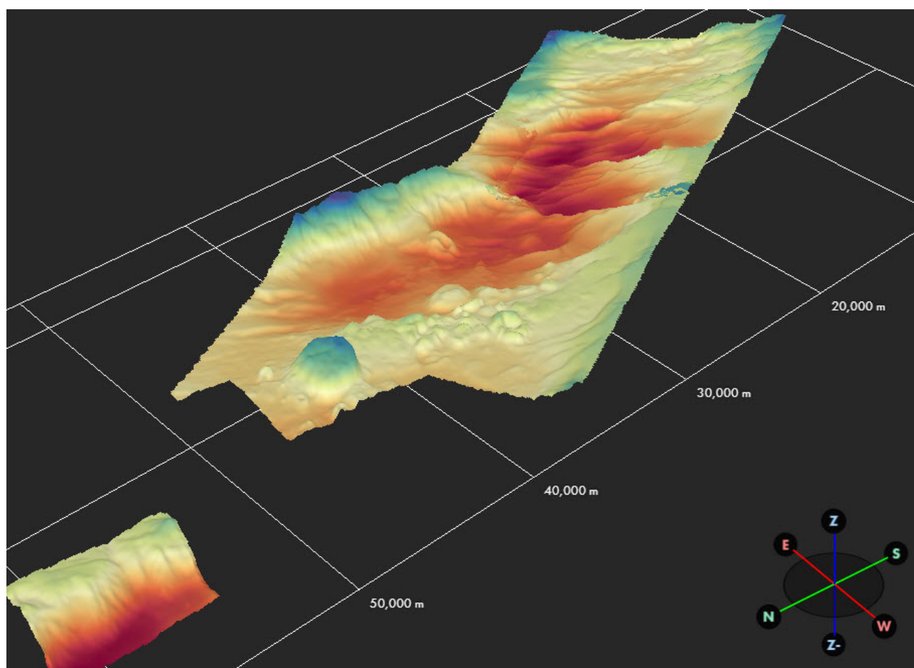
Fig. 4.1 Bathymetry grid in Argeo Scope
