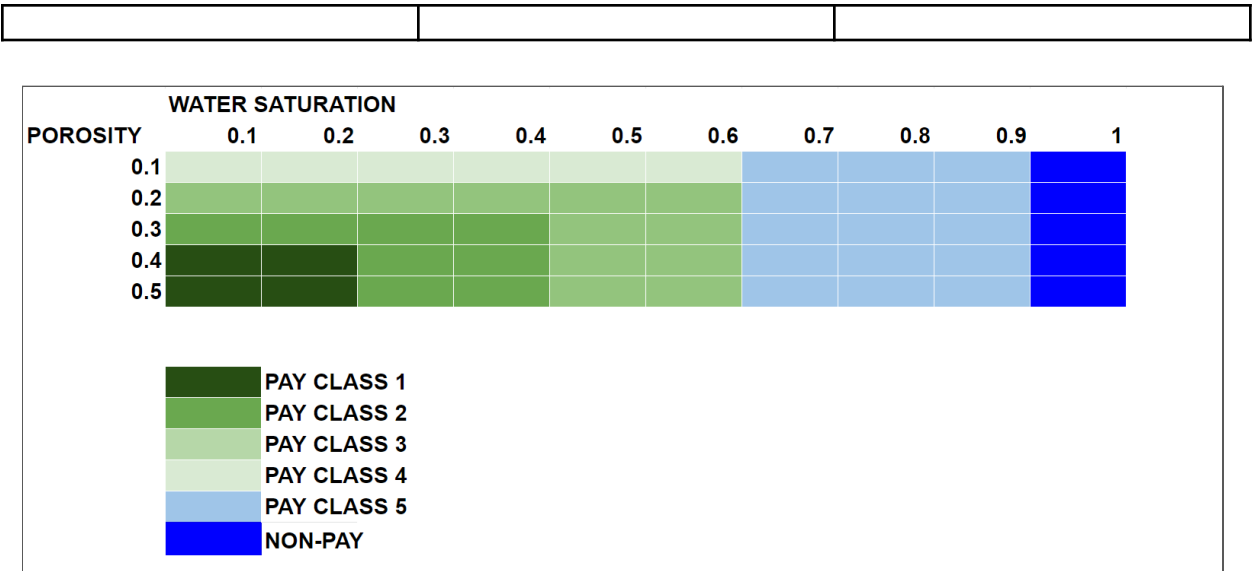
Figure 5 showing the defined pay classes based on cutoffs of Sw and porosity.
